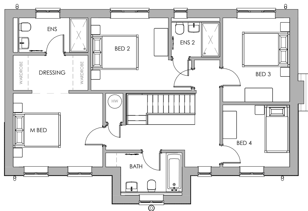
L2 First Floor Level
